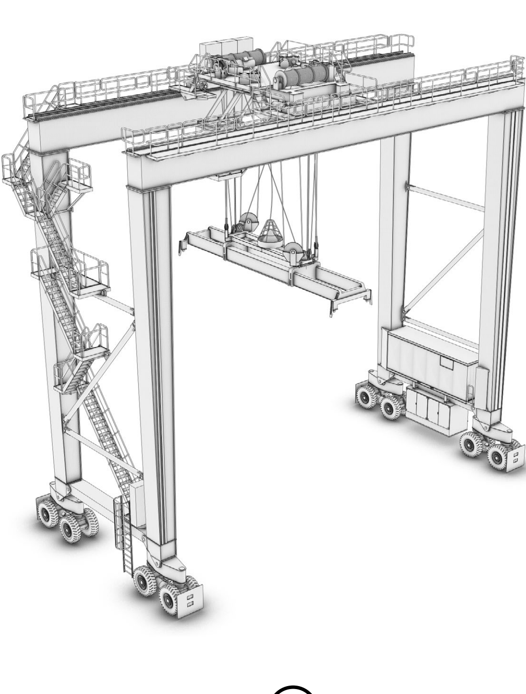
RTG Rubber-Tired Gantry Crane
