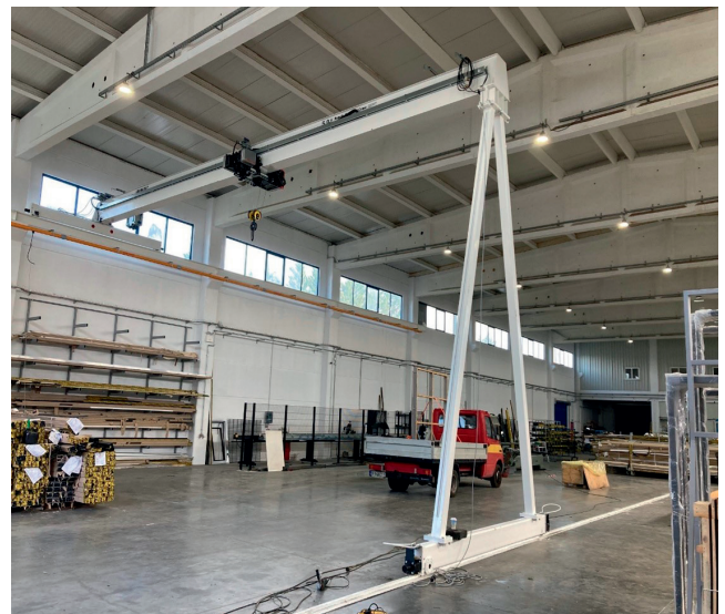
Semiportal 5 ton Single girder Crane with 14m span
