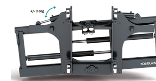
Carriage with center leveling (2 forks) for sensitive cargo
