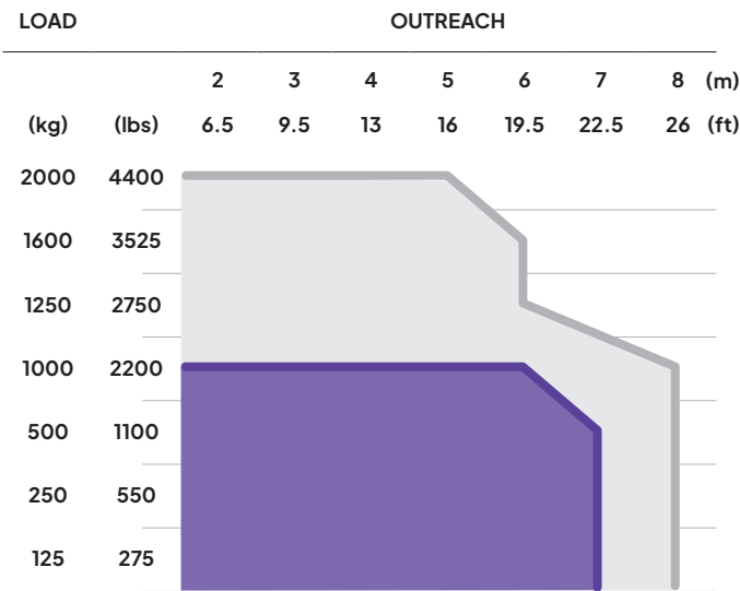
Braced, wall-mounted, I-beam with a Konecranes D-series electric chain hoist.
